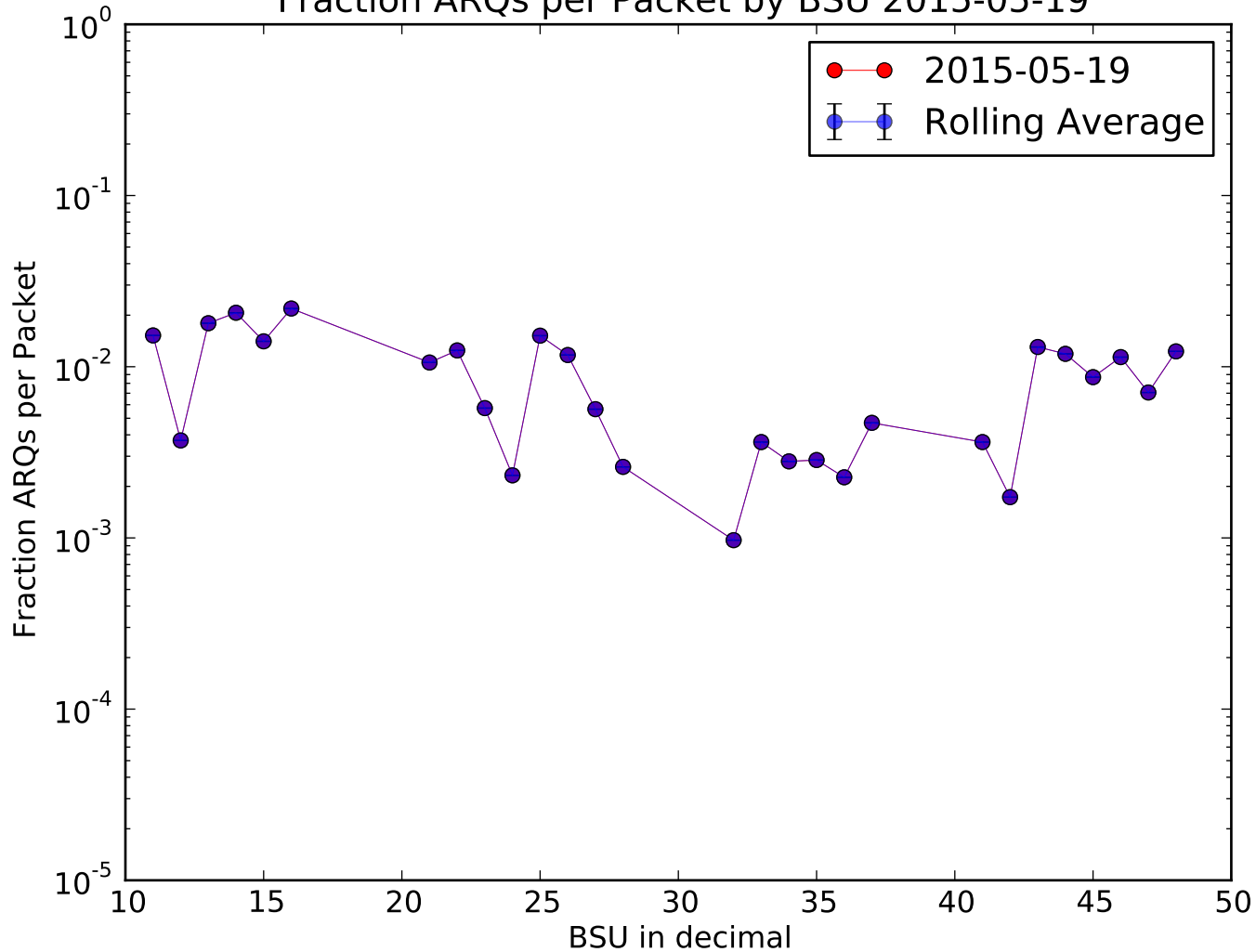
Fraction ARQs per Packet by BSU 2015-05-19
