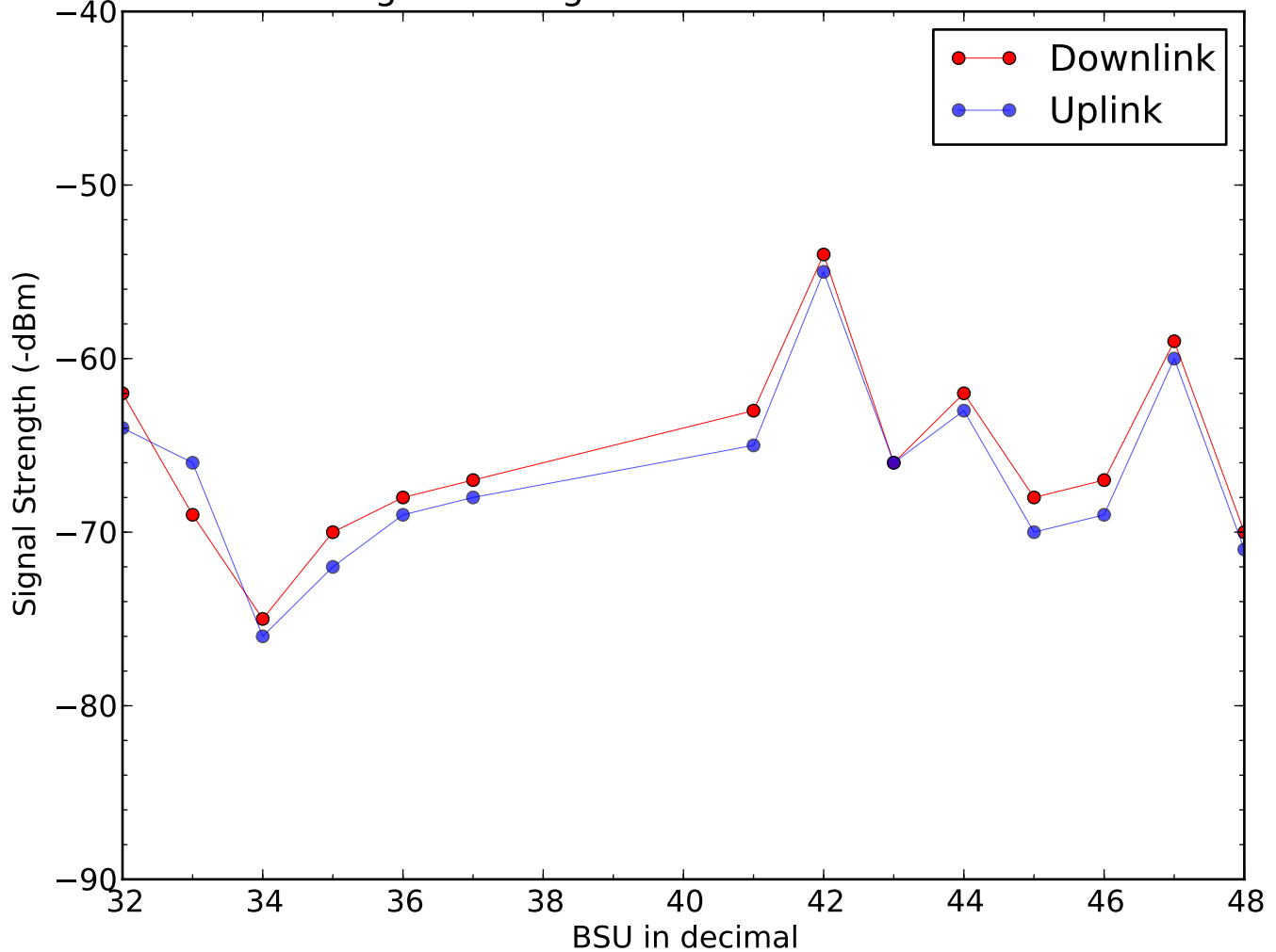
Signal Strength of BSU on 2015-05-12
