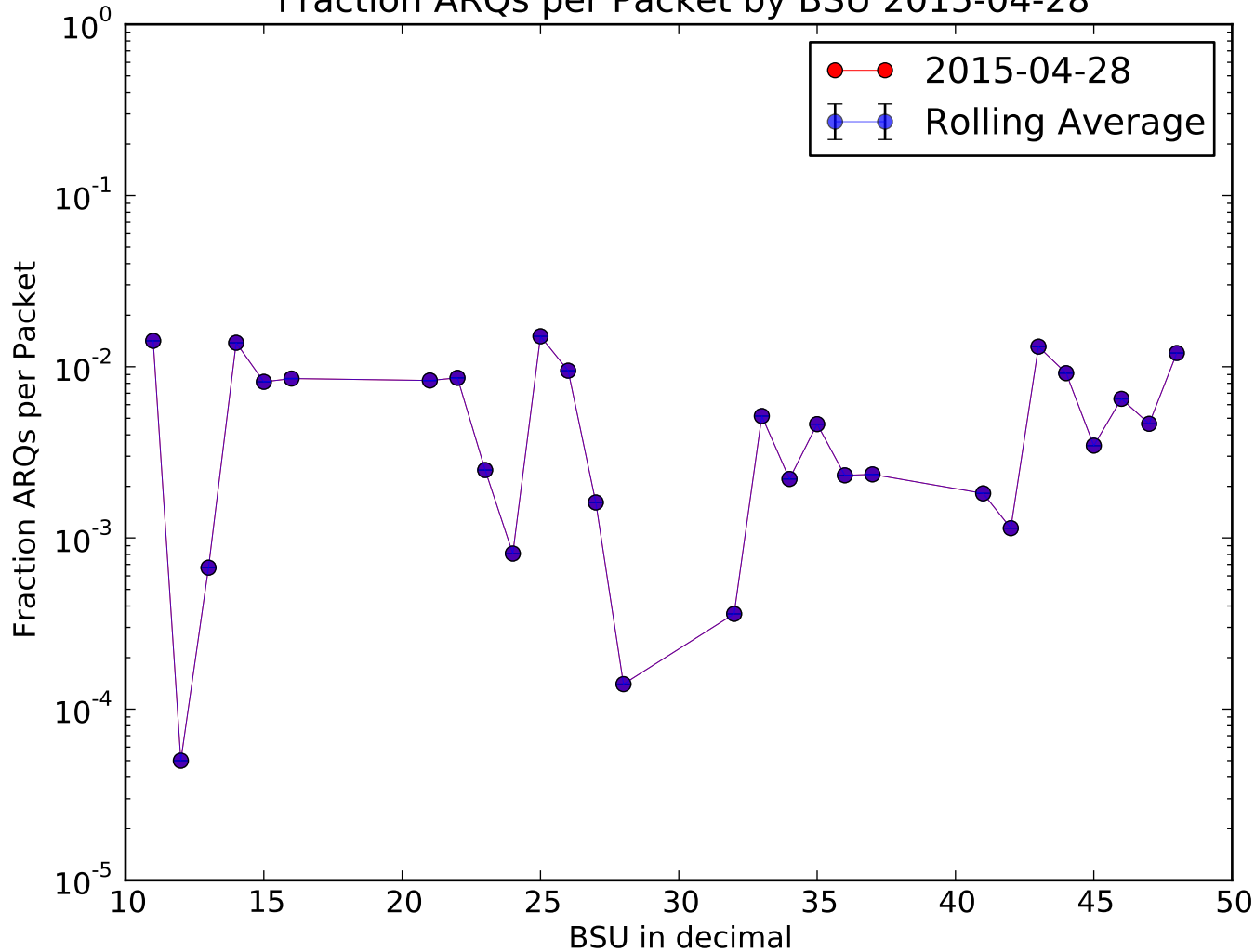
Fraction ARQs per Packet by BSU 2015-04-28
