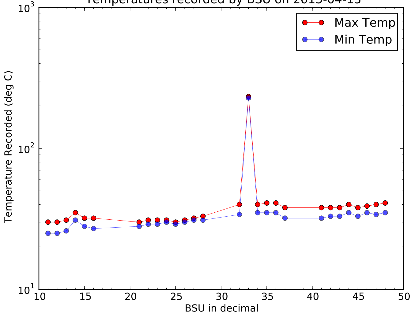
Temperatures recorded by BSU on 2015-04-13
