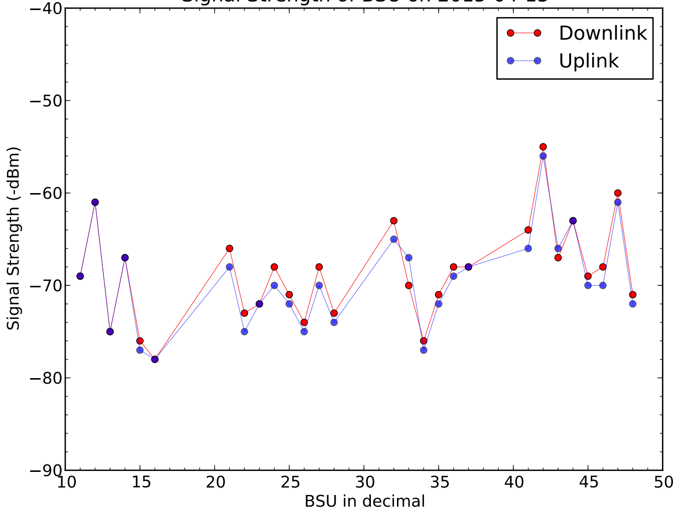
Signal Strength of BSU on 2015-04-13
