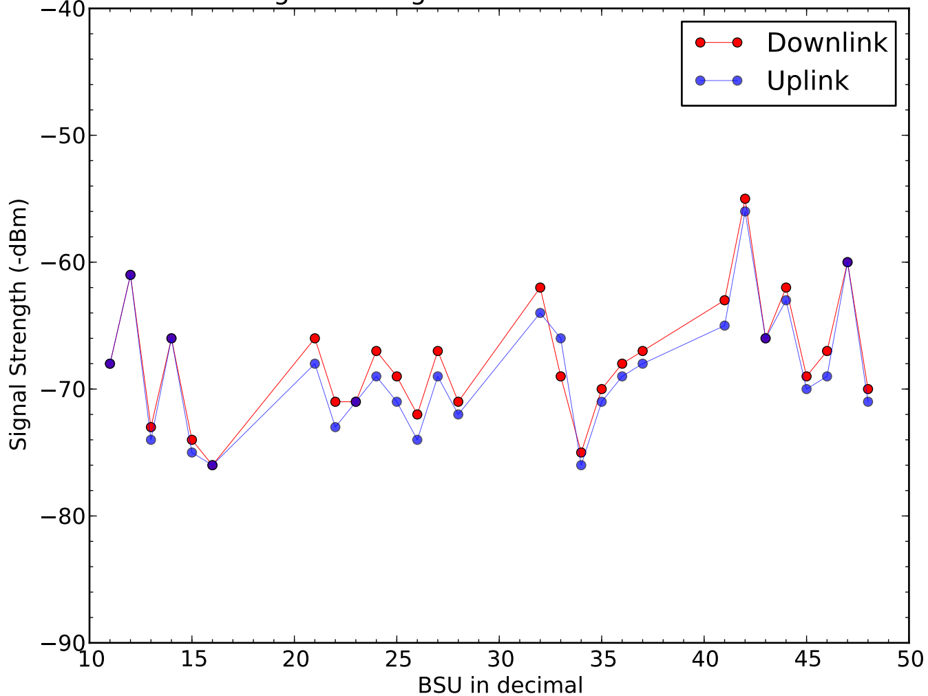
Signal Strength of BSU on 2015-04-03
