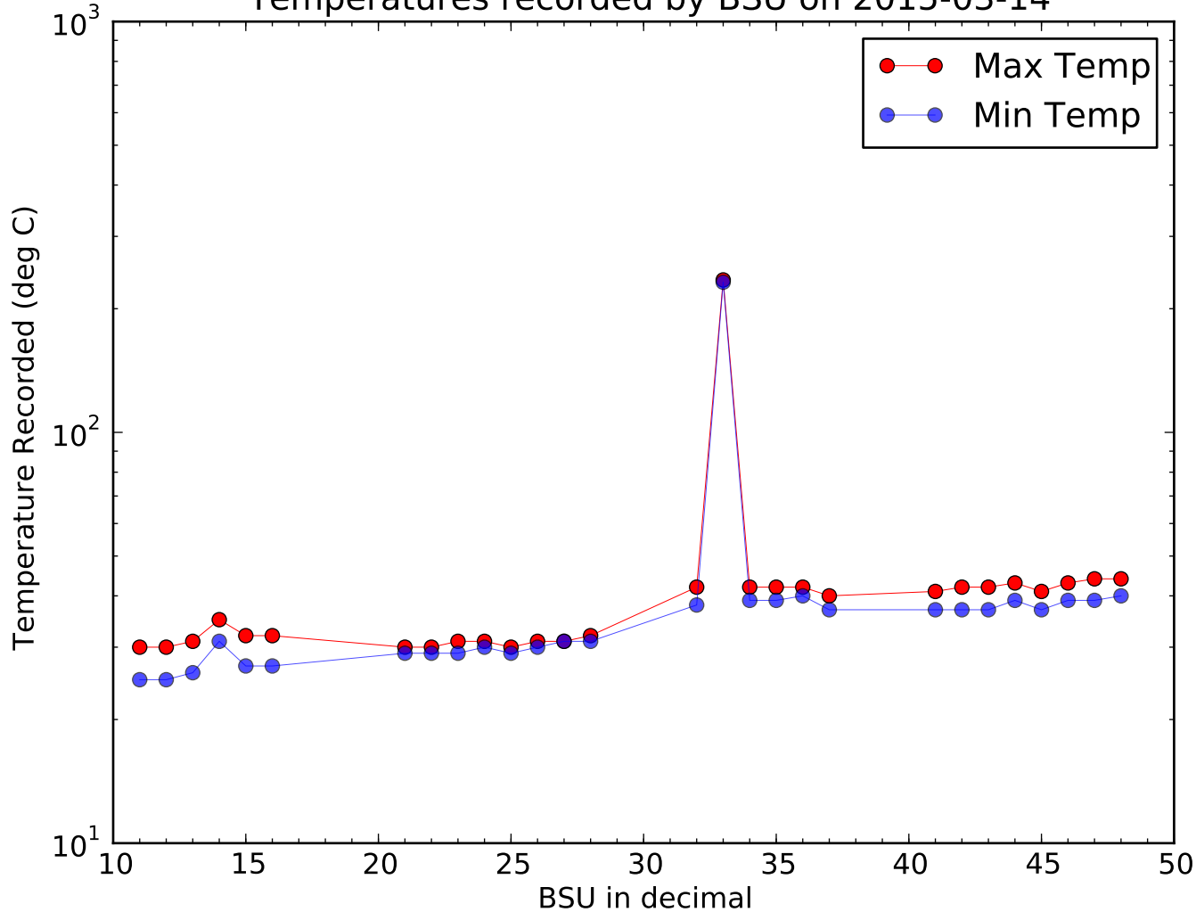
Temperatures recorded by BSU on 2015-03-14
