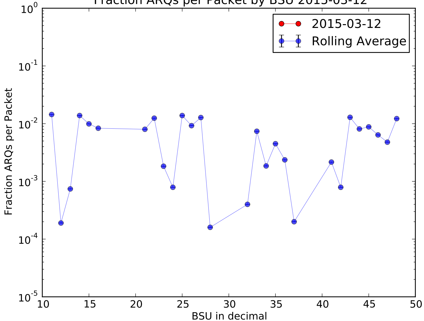
Fraction ARQs per Packet by BSU 2015-03-12
