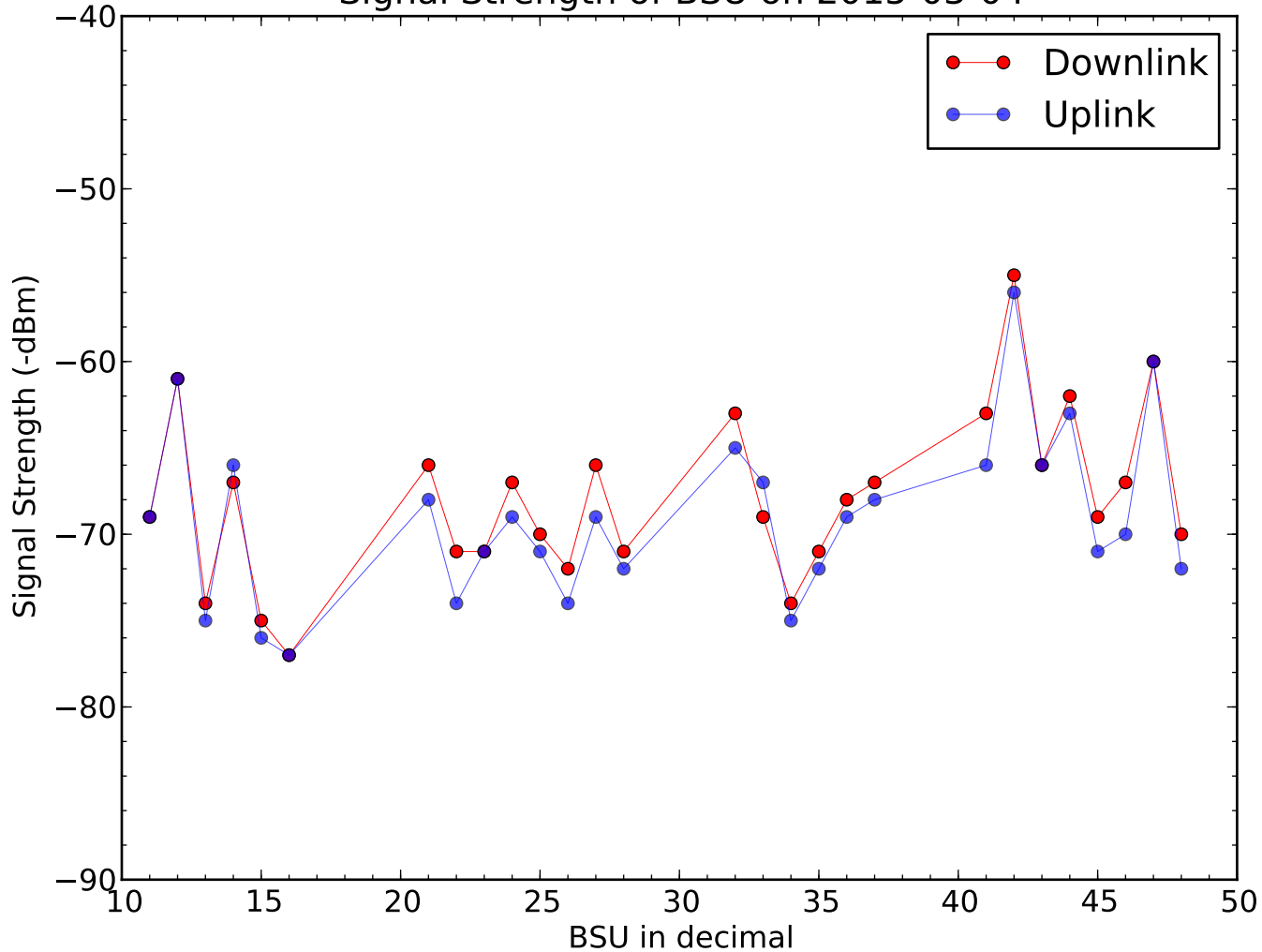
Signal Strength of BSU on 2015-03-04
