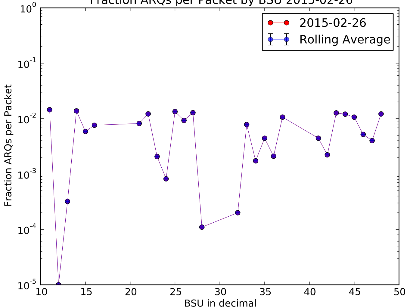
Fraction ARQs per Packet by BSU 2015-02-26
