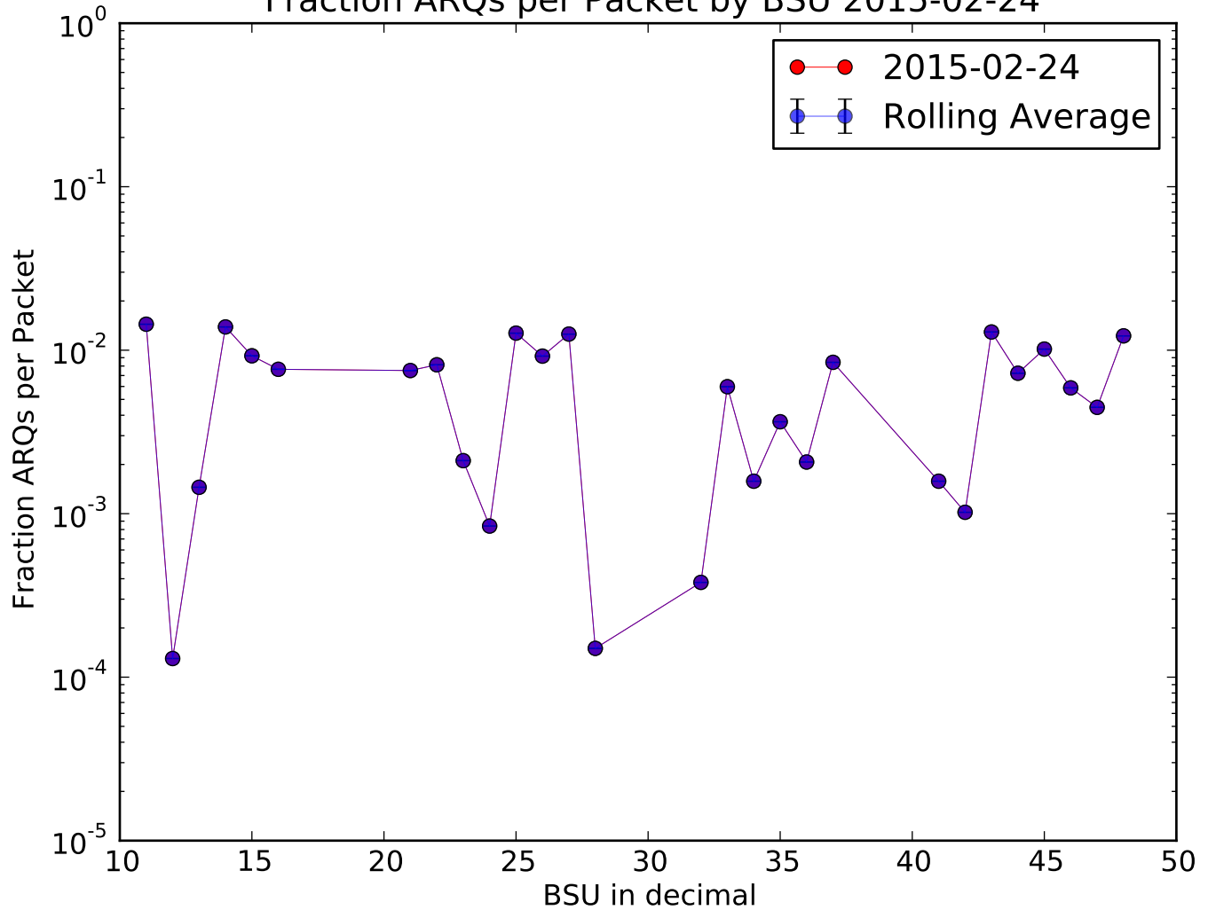
Fraction ARQs per Packet by BSU 2015-02-24
