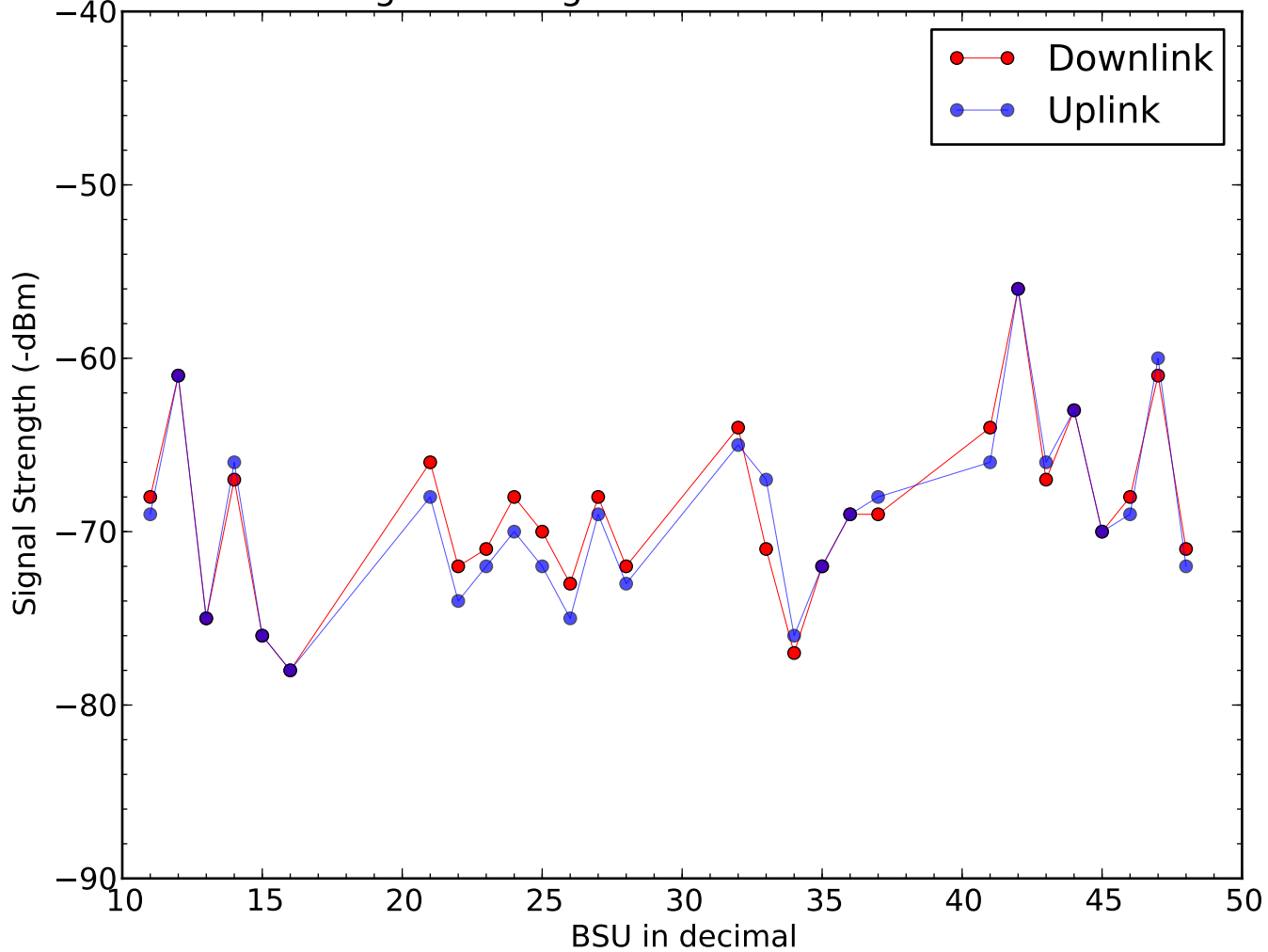
Signal Strength of BSU on 2015-02-11
