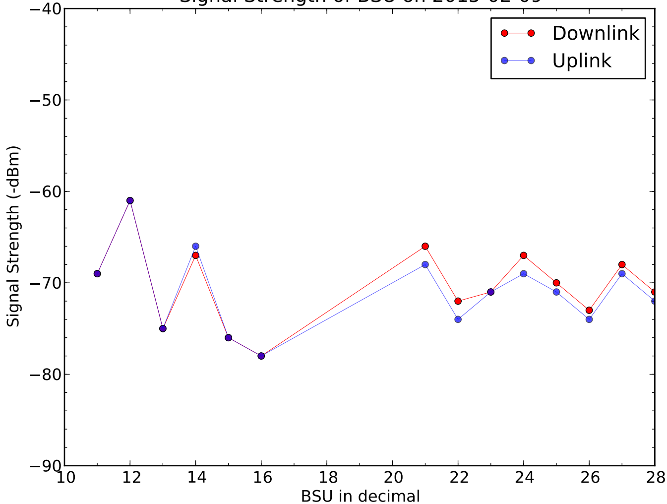
Signal Strength of BSU on 2015-02-09
