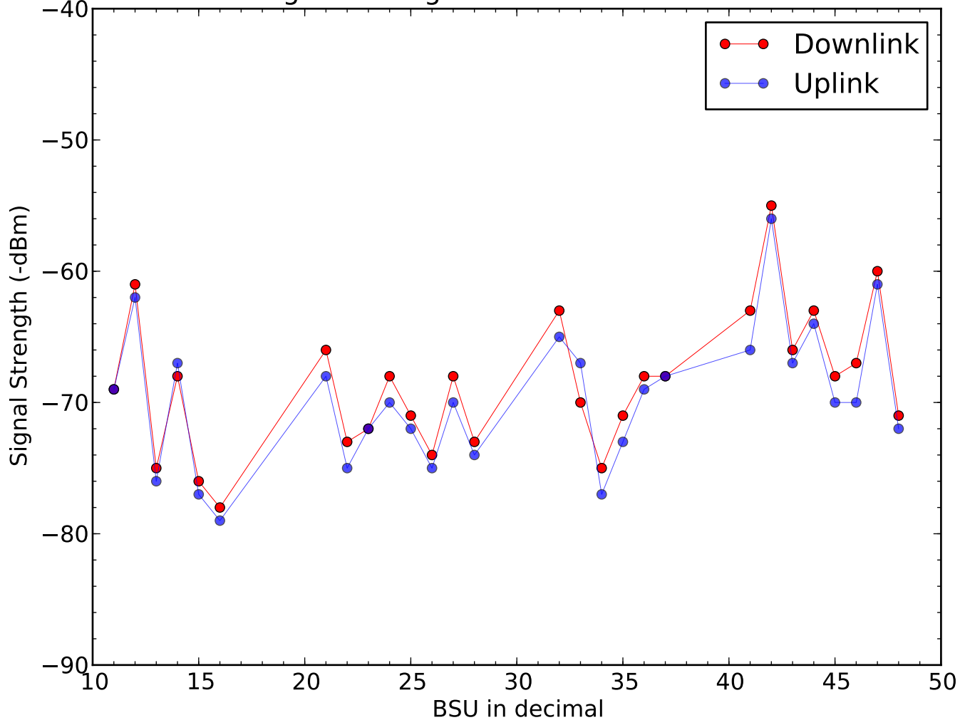
Signal Strength of BSU on 2015-02-04
