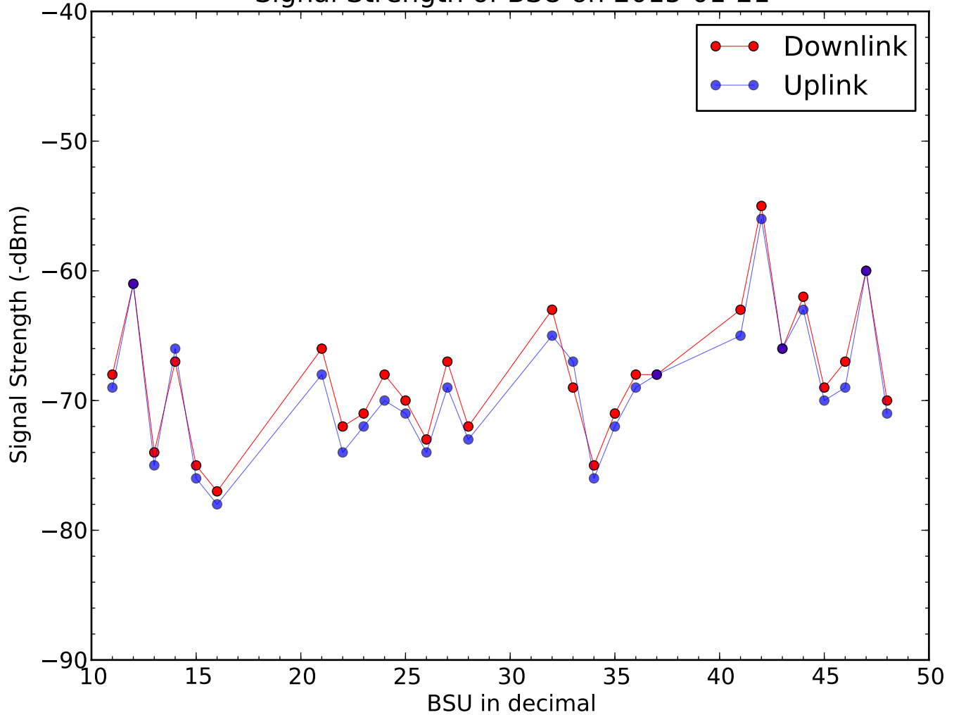
Signal Strength of BSU on 2015-01-21
