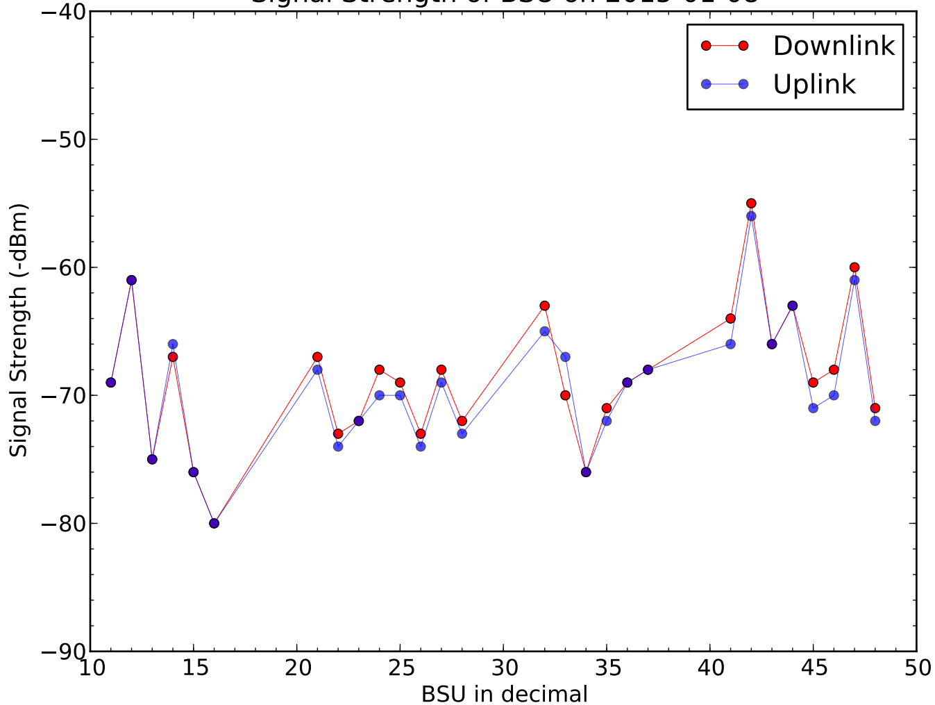
Signal Strength of BSU on 2015-01-08
