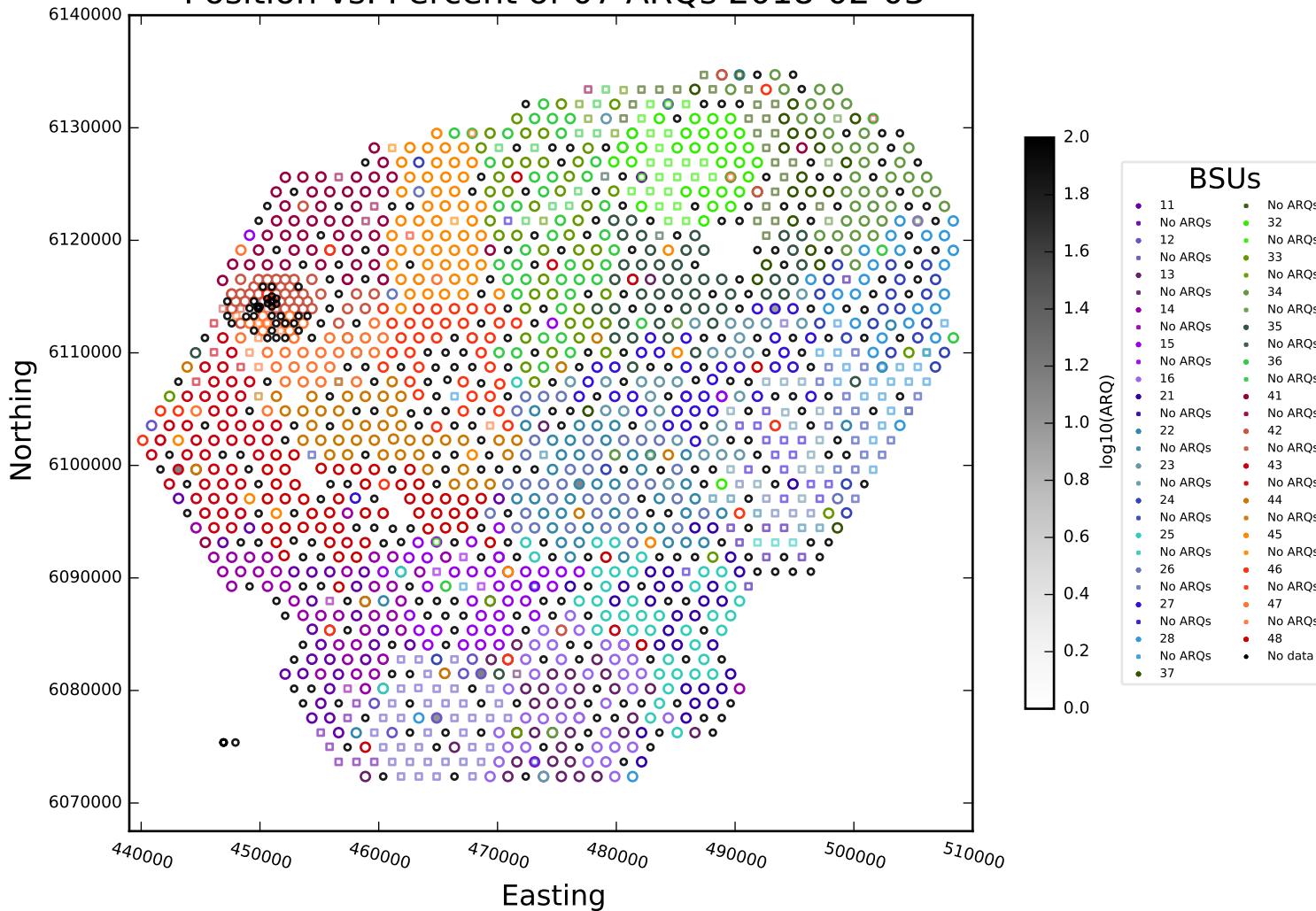
Position vs. Percent of 07 ARQs 2018-02-03
