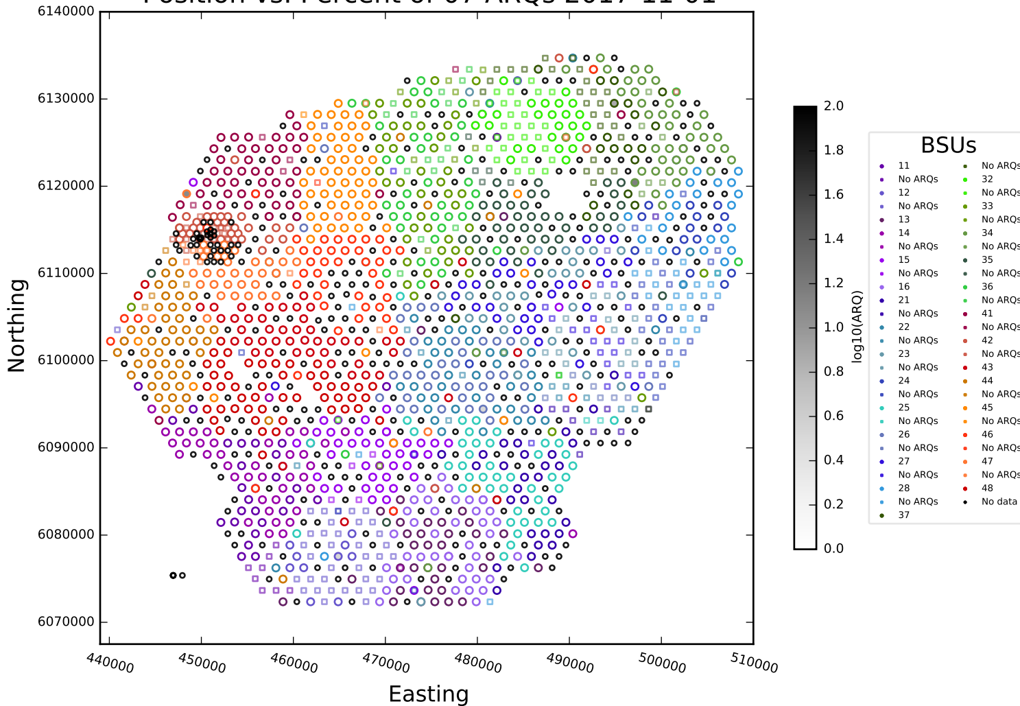
Position vs. Percent of 07 ARQs 2017-11-01
