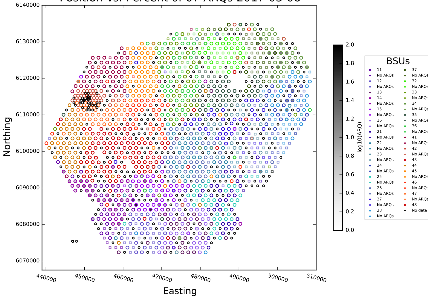
Position vs. Percent of 07 ARQs 2017-03-06
