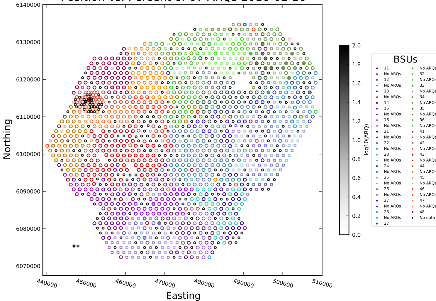
Position vs. Percent of 07 ARQs 2016-02-20
