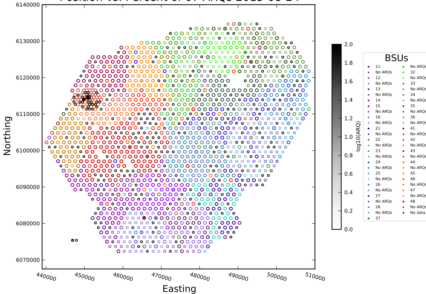
Position vs. Percent of 07 ARQs 2015-08-24
