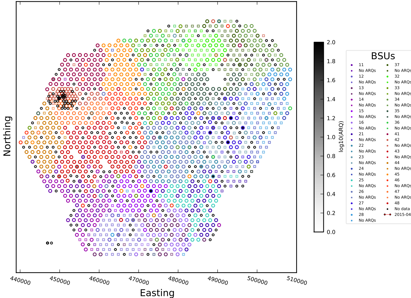
Position vs. Percent of 07 ARQs 2015-04-04
